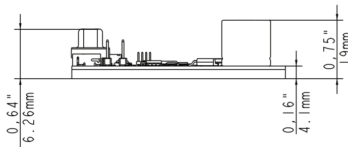
FIGURE 14. SDC2130/SDC2160 front view and dimensions
