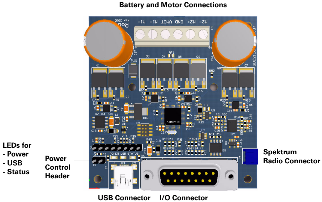
FIGURE 8. Controller layout
