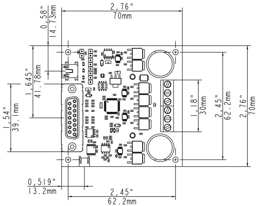
FIGURE 15. SDC2130/SDC2160 top view and dimensions
