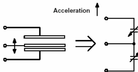
Figure II.1 Equivalent accelerometer model
